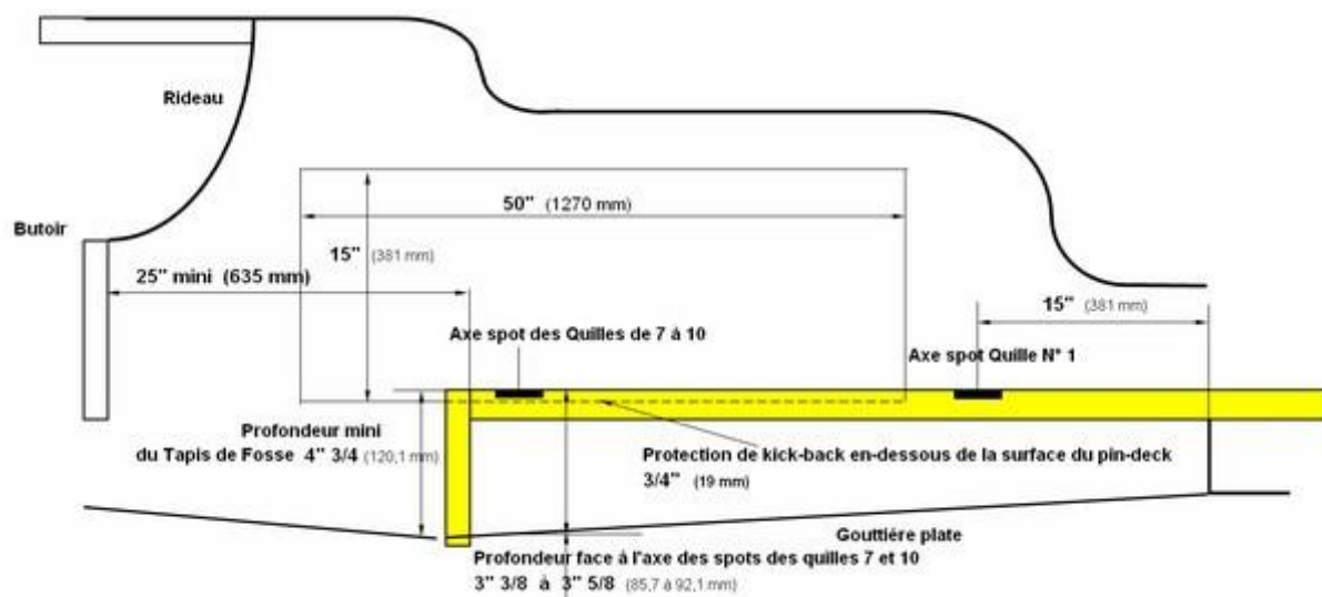
Figure 4 – Pin-deck
